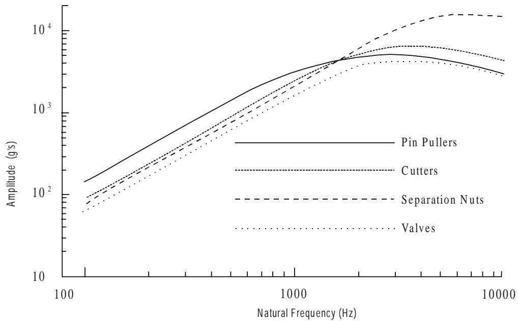
FIGURE 517-10. Shock response spectra for various point source pyrotechnic devices.
