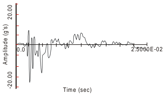
a. a_1(t) - Deterministic Signal
